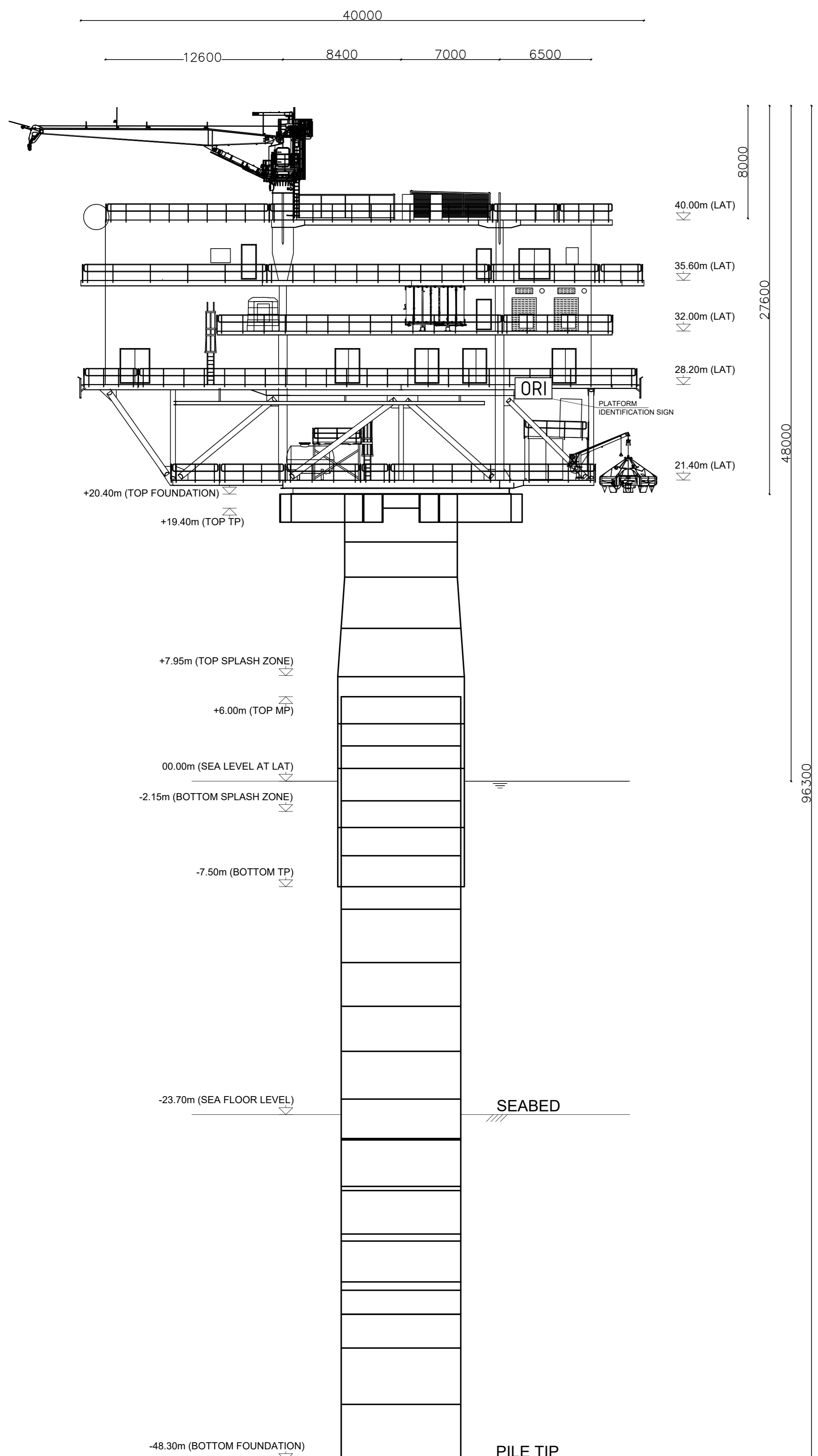
SIDE VIEW (LEFT)
